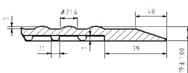
ergolastec oil_wet
